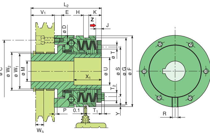
Dimensioni / overall dimensions (mm)
