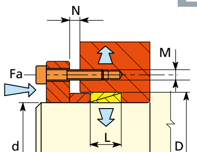
montaggio / mounting position
